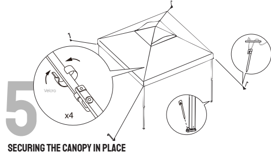
5 SECURING THE CANOPY IN PLACE
